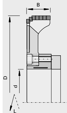
Hogger on hydro bushing 183821 - saw blade away from the spindle (version 1)
