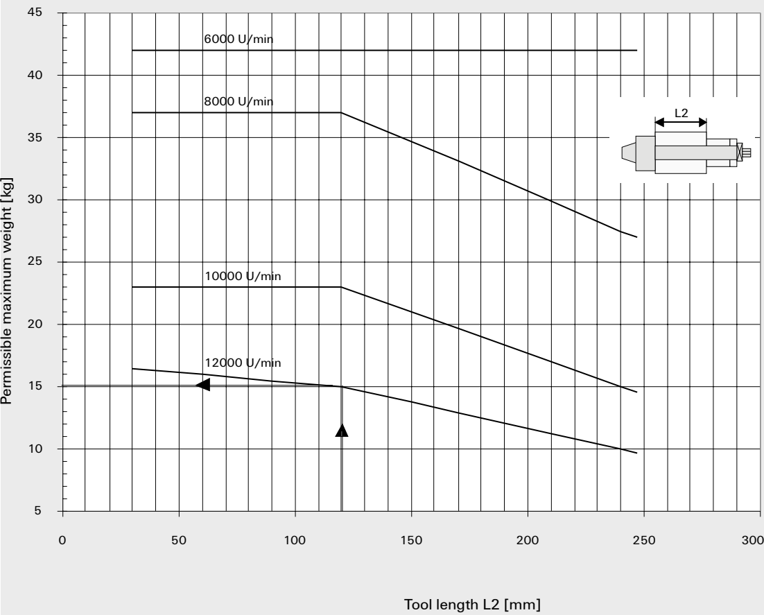
Diagram for PowerLock-Adapter
