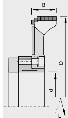
Hogger on hydro bushing 183821 - saw blade towards the spindle (version 2)
