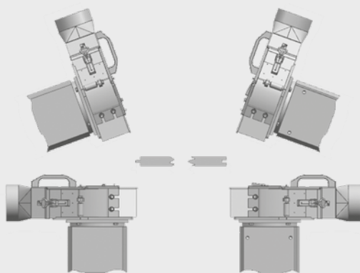
T1602 dust hood with fixed cover
